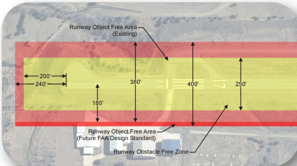
FIGURE 3-6 RUNWAY 17 OFZ/OFA – EXISTING AND STANDARD RALPH M. HALL MUNICIPAL AIRPORT
