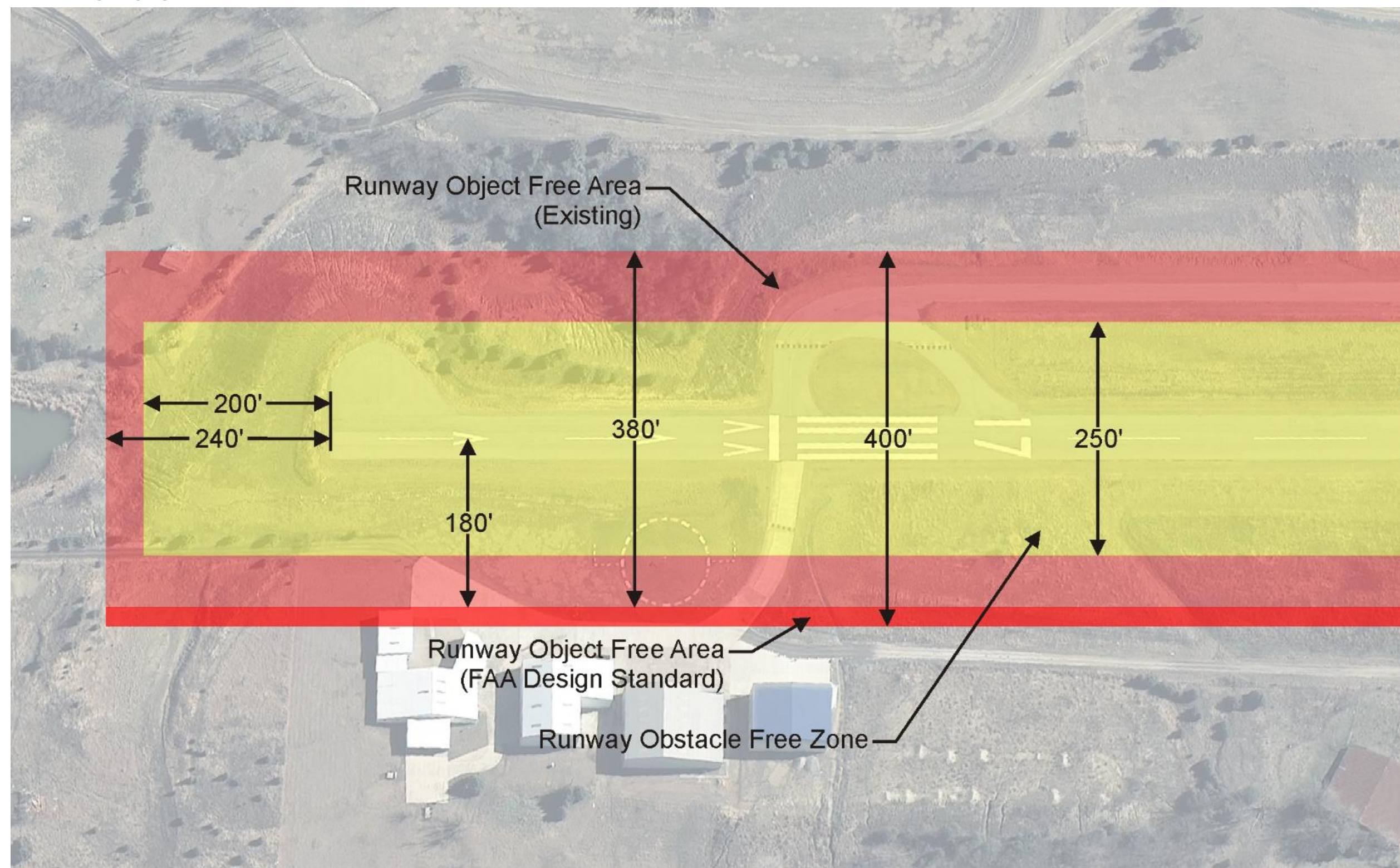
FIGURE 4-3 RUNWAY 17 DEFICIENCIES
