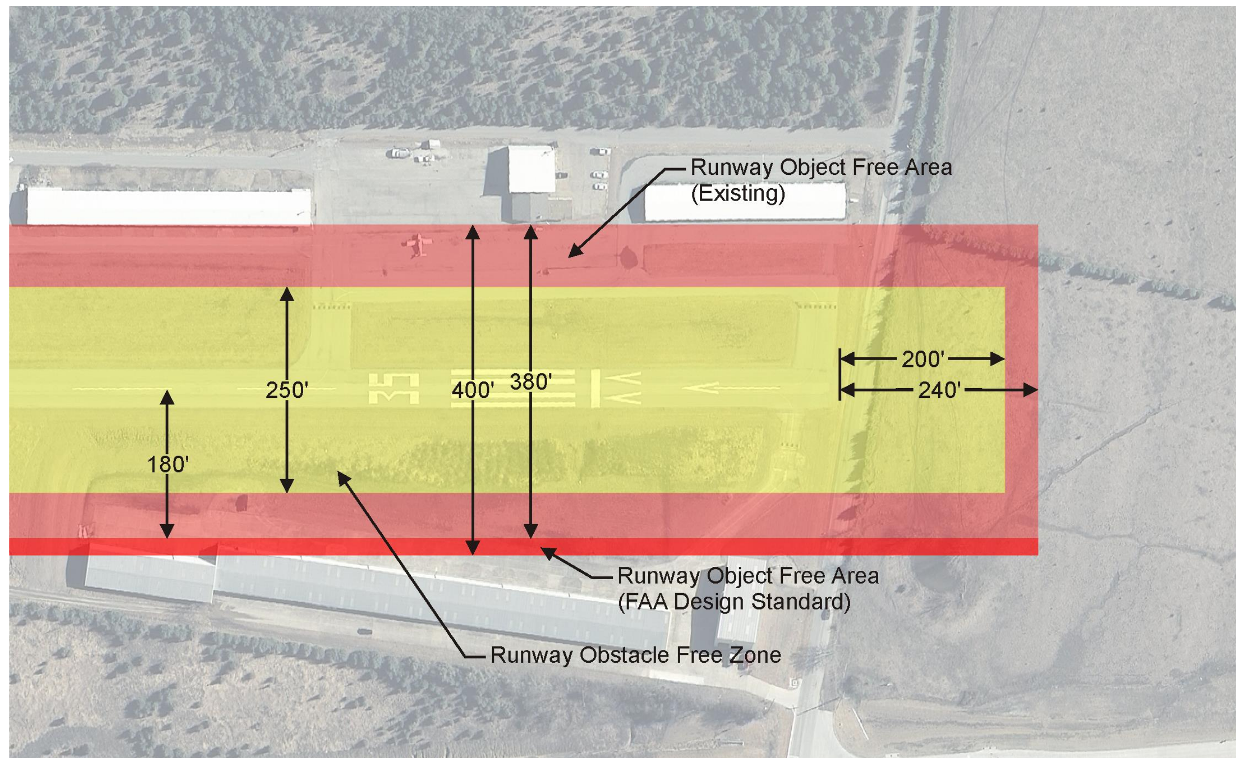
FIGURE 4-4 RUNWAY 35 DEFICIENCIES
